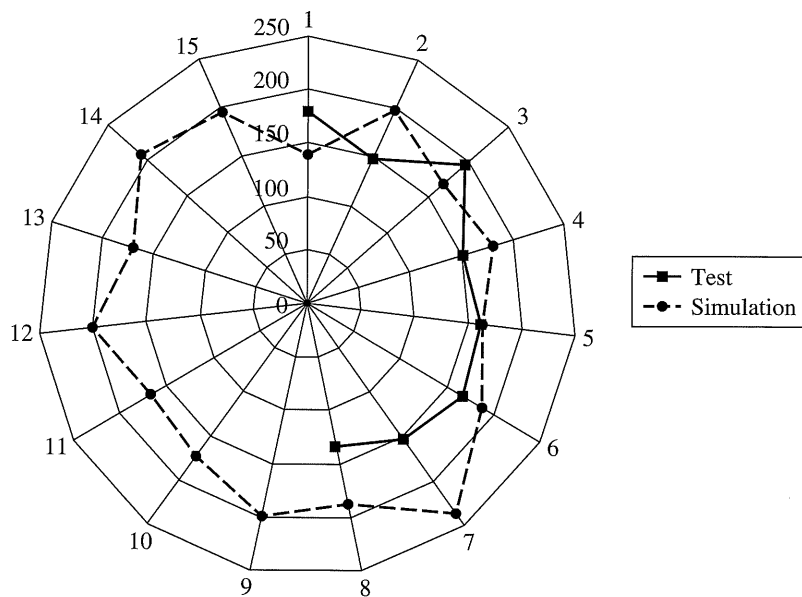
FIGURE 5.3 Spider-web plot for the missile and simulation miss distances.
